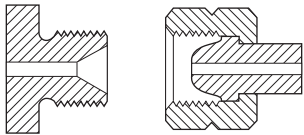
CGA 290 .745-14NGO-LH-EXT
