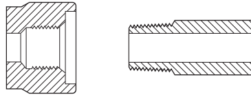
CGA 240 .375-18NGT-RH-INT
