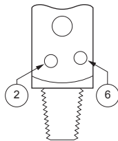
CGA 880 Pin-Indexed Yoke, Pins 2-6
