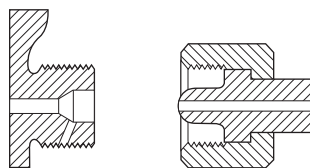
CGA 326 .825-14NGO-RH-EXT (Small Round Nipple)
