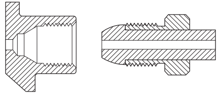
CGA 296 .803-14UNS-2B-RH-INT
