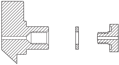
CGA 110 .3125-32UNEF-2B-RH-INT
