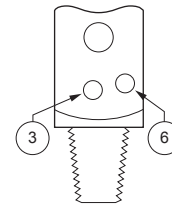
CGA 920 Pin-Indexed Yoke, Pins 3-6
