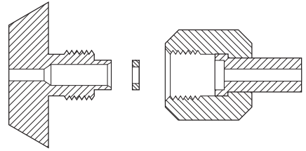
CGA 280 .745-14NGO-RH-EXT
