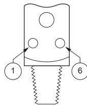
CGA 940 Pin-Indexed Yoke, Pins 1-6
