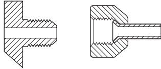
Standard Thermal Platform Inlet
