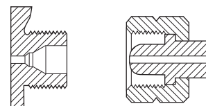
CGA 350 .825-14NGO-LH-EXT (Round Nipple)
